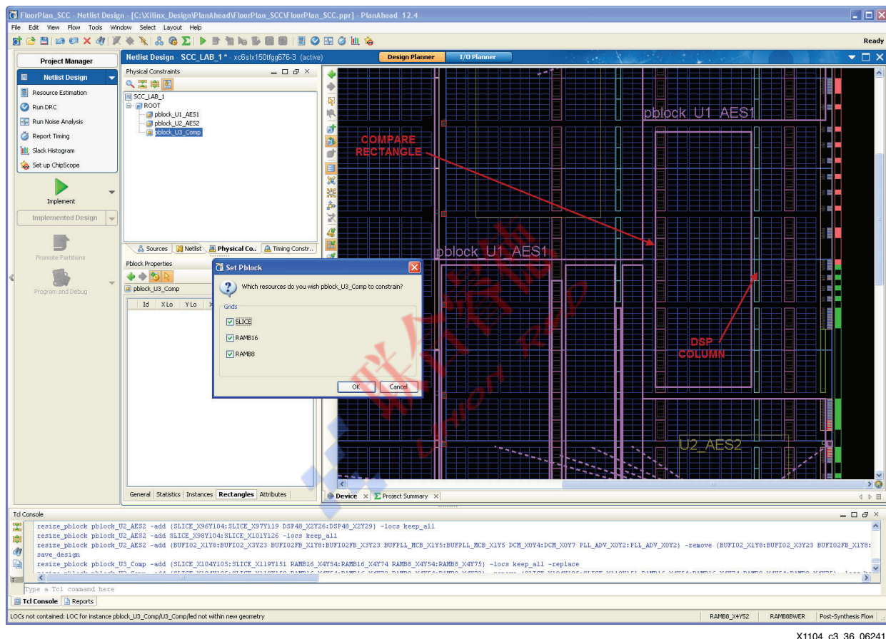
Figure 3-36: pblock_U3_Comp Pblock Layout (Set Pblock)
