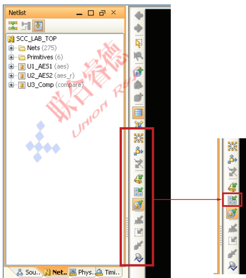
Figure 3-7: Select Site Constraint Mode Symbol
