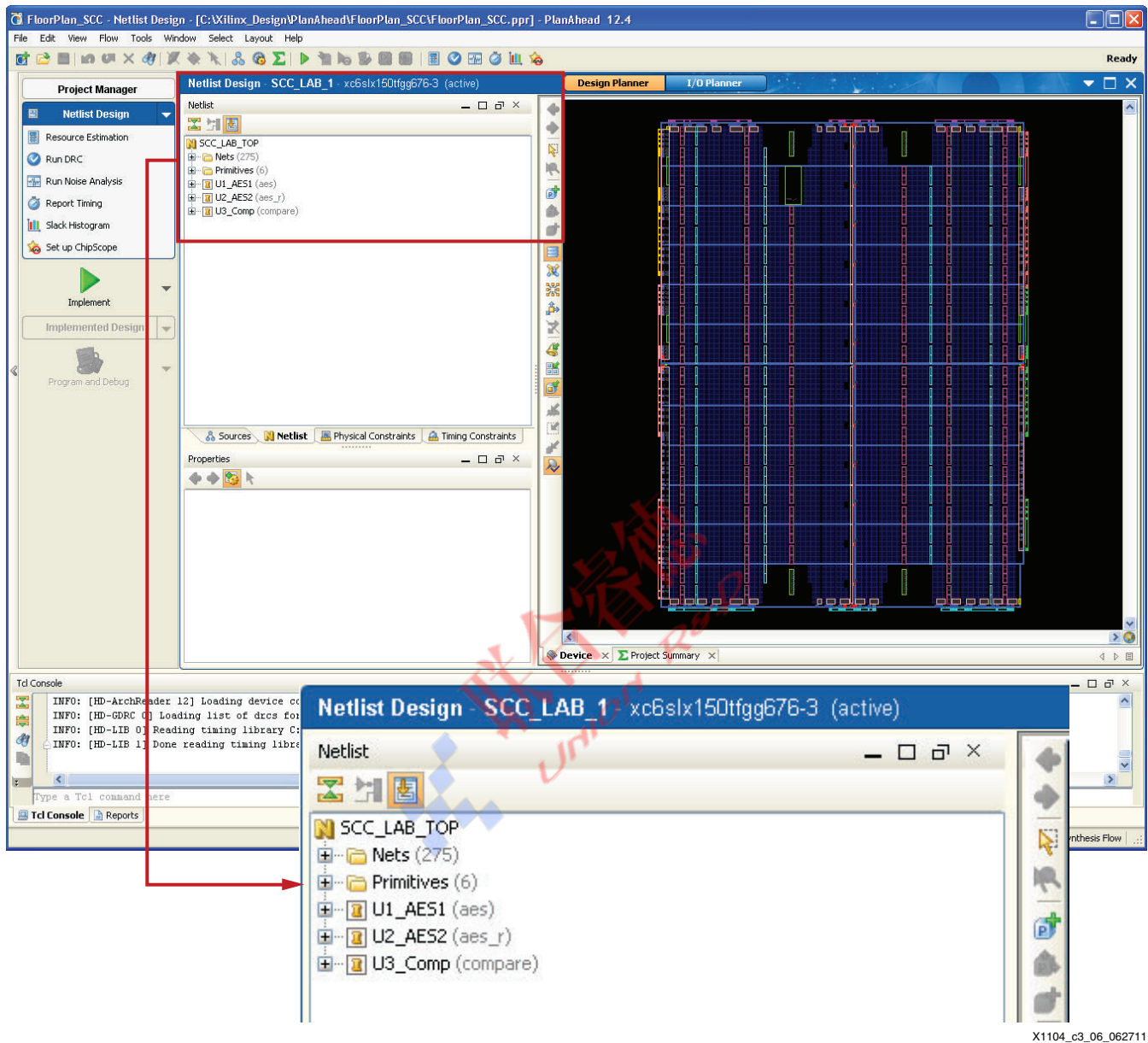
Figure 3-6: PlanAhead Design Planner View
