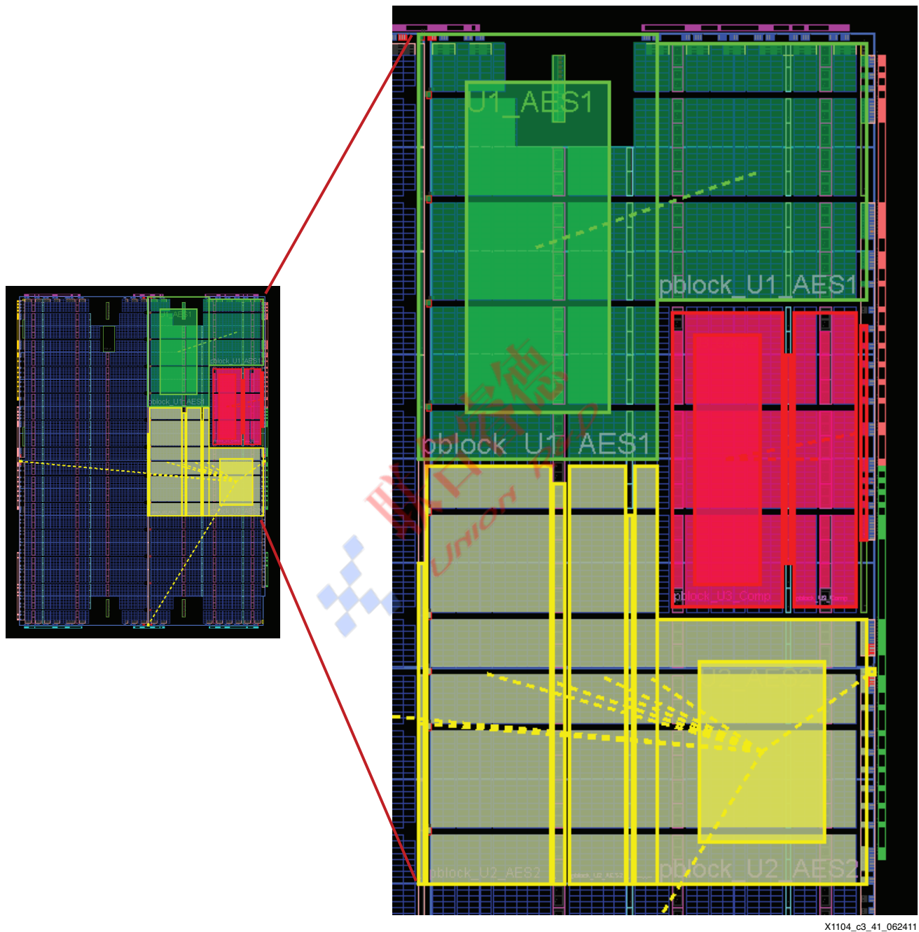
Figure 3-41: Final Layout
