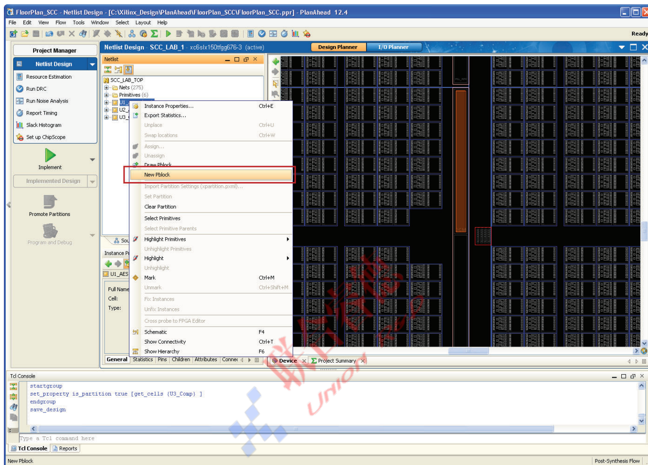
Figure 3-19: New Pblock
